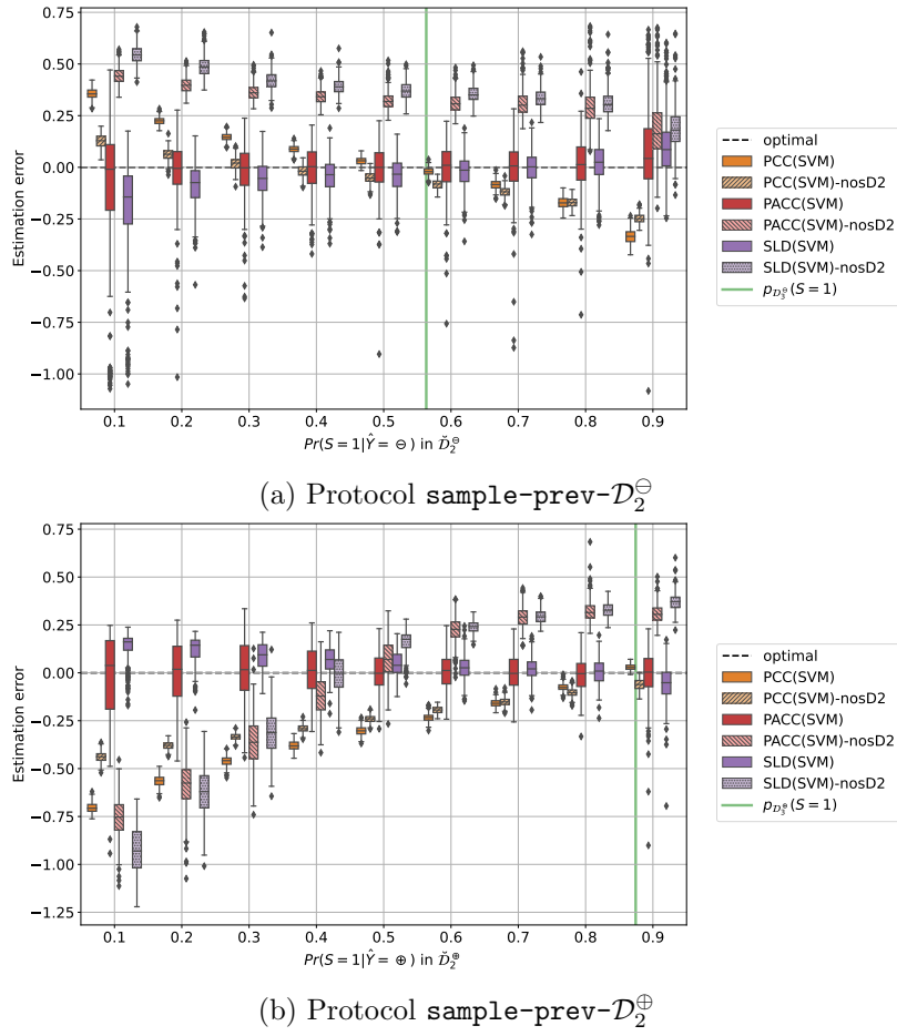
Figure 10: Results obtained in the ablation study on the Adult dataset with SVM-based quantification for protocol sample-prev- \mathcal{D}_2 .
