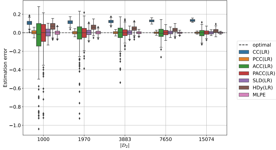
Figure 3: Protocol sample-size- \mathcal{D}_2 on the Adult dataset. Distribution of the estimation error ( y axis) as the cardinality |\mathcal{D}_2| is varied ( x axis).
