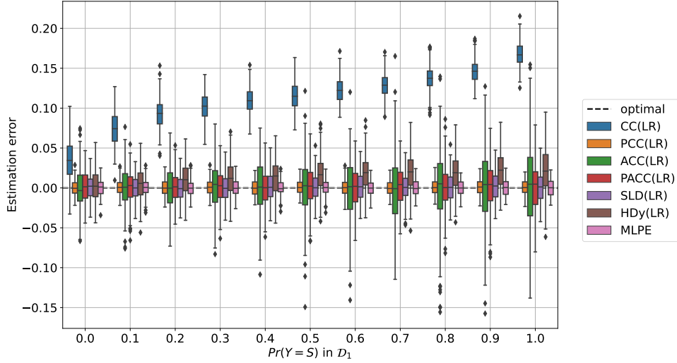
Figure 4: Protocol sample-prev- \mathcal{D}_1 on the Adult dataset. Distribution of the estimation error ( y axis) as \tilde{\mathcal{D}}_1 is sampled with a given \Pr(Y = S) ( x axis). Each boxplot summarizes the results of 5 random splits, 6 role permutations and 10 samplings of \tilde{\mathcal{D}}_1 .
