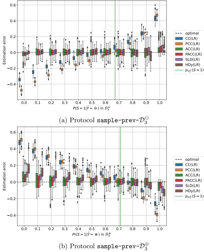
Figure 6: Experiments conducted according to protocol \text{sample-prev-}\mathcal{D}_3 on a fairness-aware classifier.
