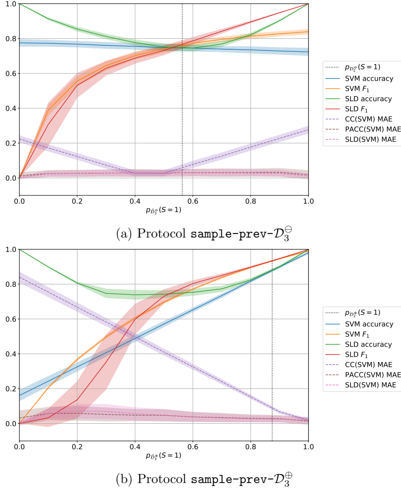
Figure 13: Performance of SVM-based methods CC, SLD and PACC on the Adult dataset when used for quantification (MAE – lower is better) and classification ( F_1 , accuracy – higher is better) under protocol \text{sample-prev-}\mathcal{D}_3 . The classification performance of PACC is equivalent to that of CC (both equal to the performance of the underlying SVM), and we thus omit it for readability.
